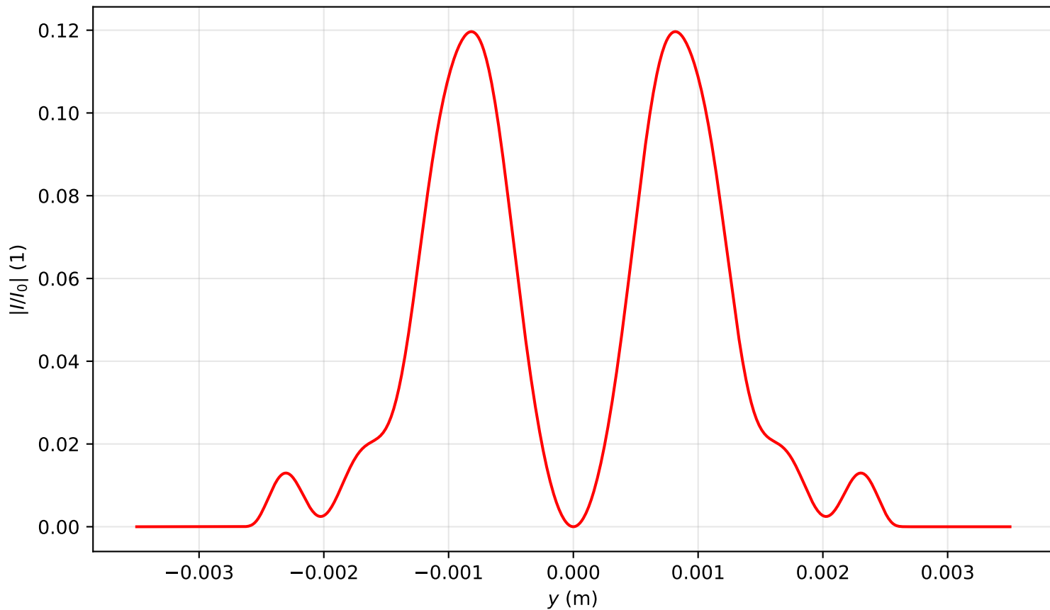
Intensity profile I(x=0, y, z=3.503)/I_0 , \text{Pin}=4.0\text{Pcr} , artificial time
